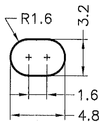
HOLE IN P.C.B P.C.B THICKNESS:1.57mm
