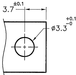
HOLE IN P.C.B P.C.B THICKNESS:1.57mm
