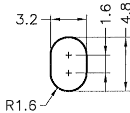
HOLE IN P.C.B P.C.B THICKNESS:2.13mm
