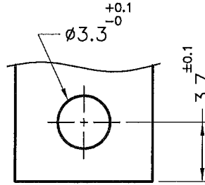
HOLE IN P.C.B P.C.B THICKNESS:1.57mm
