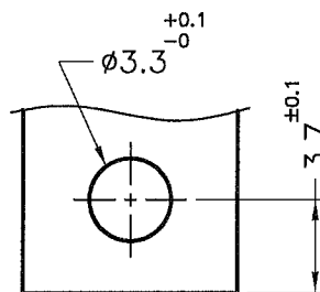
HOLE IN P.C.B P.C.B THICKNESS:1.57mm
