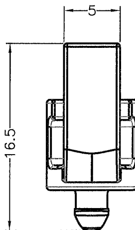
HOLE IN P.C.B P.C.B THICKNESS:1.57mm
