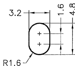
HOLE IN P.C.B P.C.B THICKNESS:1.57mm
