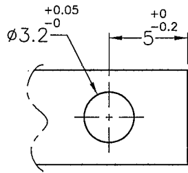
HOLE IN P.C.B THICKNESS: 1.6±0.2mm
