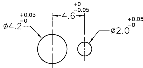
HOLE IN P.C.B THICKNESS: 1.93±0.2mm
