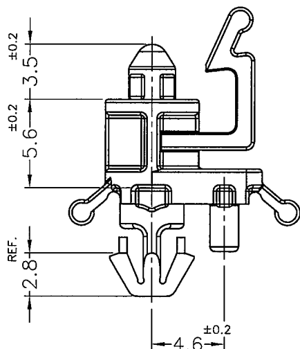
HOLE IN P.C.B THICKNESS: 1.4~1.8mm
