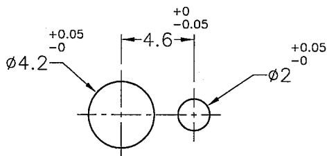
HOLE IN P.C.B THICKNESS: 2.3~2.7mm
