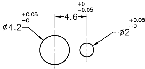
HOLE IN P.C.B THICKNESS: 2.52~3.23mm (RECOMMEND FOR REFERENCE ONLY)
