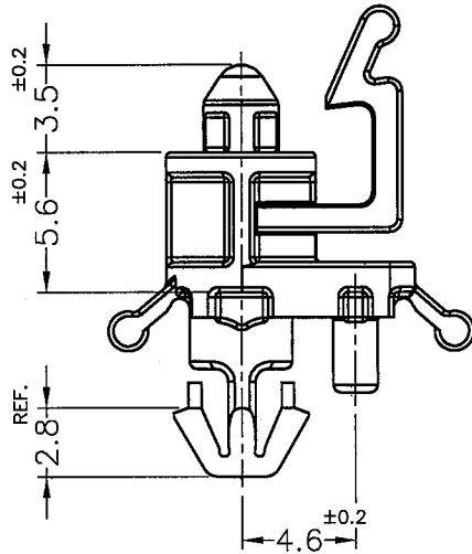
HOLE IN P.C.B THICKNESS: 1.4~1.8mm (RECOMMEND FOR REFERENCE ONLY)
