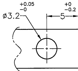
HOLE IN P.C.B THICKNESS: 1.4~1.8mm (RECOMMEND FOR REFERENCE ONLY)
