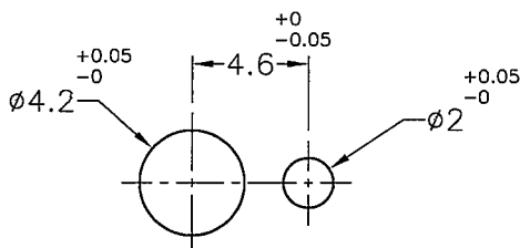
HOLE IN P.C.B THICKNESS: 2.83~3.47mm
