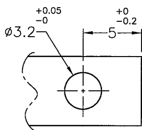
HOLE IN P.C.B THICKNESS: 1.4~1.8mm
