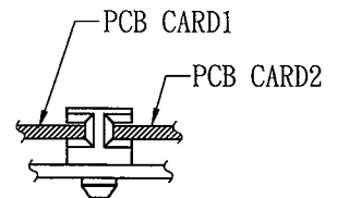
INSTALLATION DIAGRAM (安裝示意圖) SCALE 1:1
