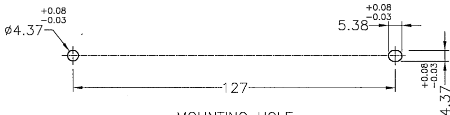
MOUNTING HOLE (RECOMMEND FOR REFERENCE ONLY)
