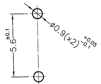
PWB LAYOUT
