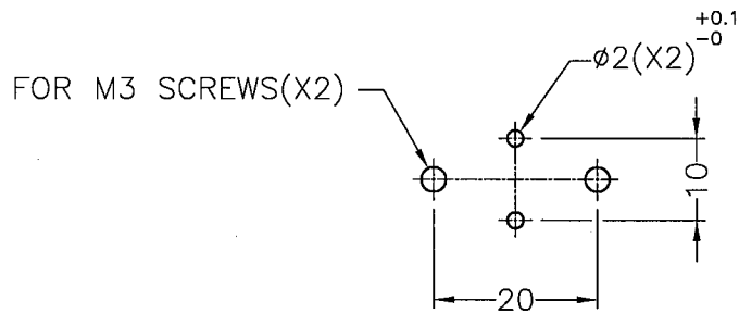
MOUNTING HOLE (RECOMMEND FOR REFERENCE ONLY)
