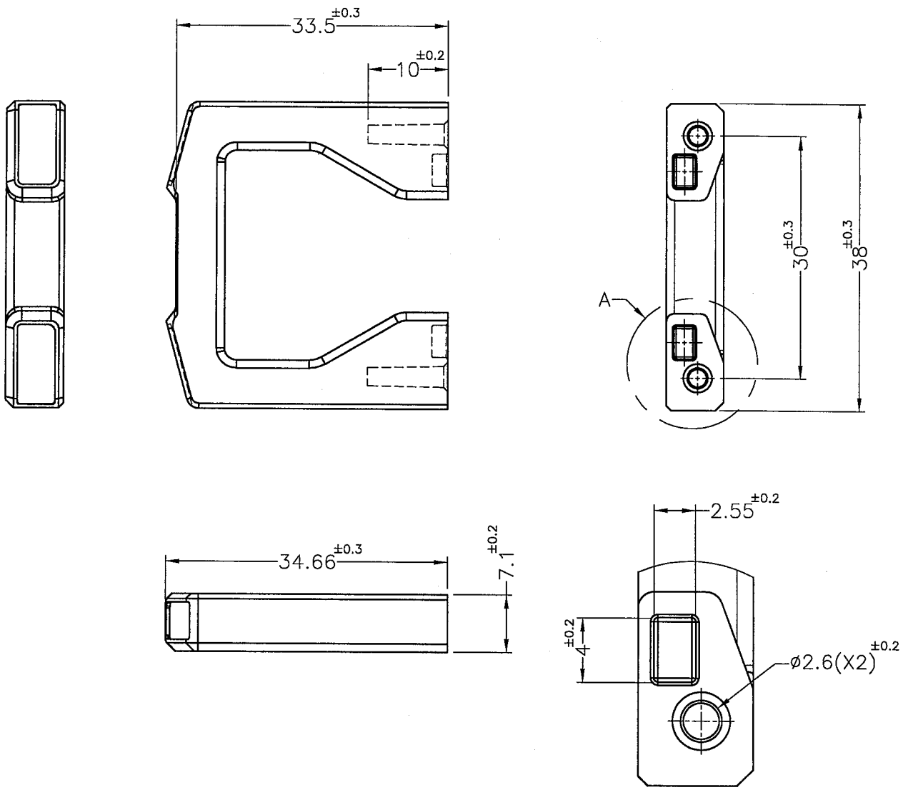
DETAIL A SCALE 3:1
