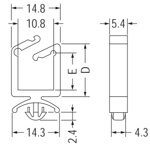
MOUNTING HOLE Ø4.8 THICKNESS 0.8-1.6
