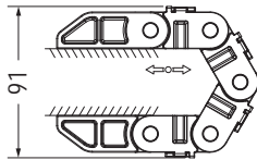
PRINCIPLE SKETCH - BEND RA-DIUS
