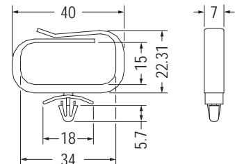
MOUNTING HOLE \varnothing 4.8\text{-}\varnothing 5.5 THICKNESS 0.8-2.0
