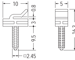
MOUNTING HOLE Ø3.0
