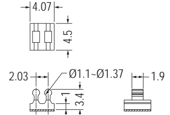
3M DOUBLE ADHESIVE TAPE
