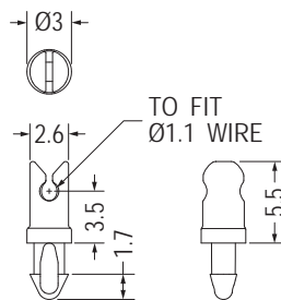
MOUNTING HOLE \varnothing 2.0 THICKNESS 1.6~2.0
