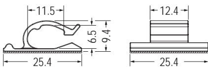
3M DOUBLE ADHESIVE TAPE
