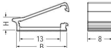
3M DOUBLE ADHESIVE TAPE
