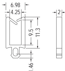
MOUNTING HOLE Ø2.8 THICKNESS 2.0
