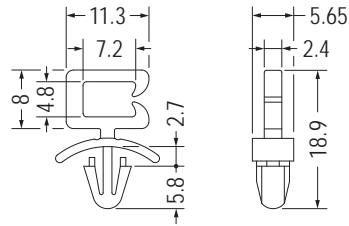
MOUNTING HOLE Ø4.8 THICKNESS 0.8-2.0
