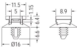
MOUNTING HOLE \varnothing 4.5\text{-}\varnothing 5.0 THICKNESS 0.8-7.0
