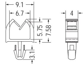
MOUNTING HOLE Ø3.0 THICKNESS 2.4
