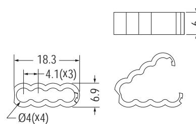
UNIT FOLDED VIEW
