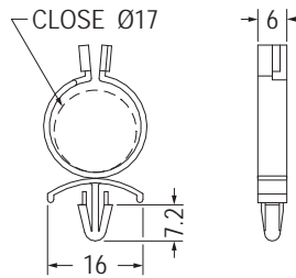
MOUNTING HOLE \varnothing 4.8 THICKNESS 1.0~3.2
