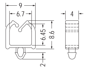
MOUNTING HOLE Ø3.0 THICKNESS 1.1
