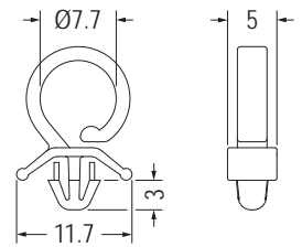
MOUNTING HOLE \varnothing 4.0 THICKNESS 0.6~2.0
