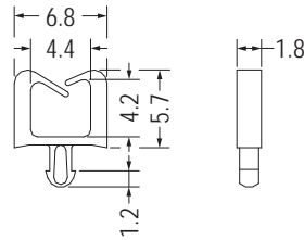
MOUNTING HOLE Ø1.75 THICKNESS 1.6
