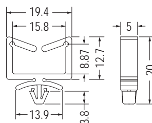
MOUNTING HOLE Ø4.5 THICKNESS 0.8-1.0
