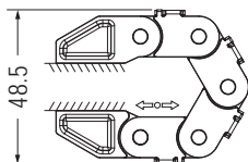
PRINCIPLE SKETCH - BEND RA-DIUS
