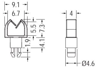
MOUNTING HOLE Ø3.8 THICKNESS 1.6
