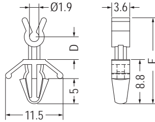
MOUNTING HOLE Ø4.0 THICKNESS 0.8-2.5
