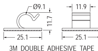
3M DOUBLE ADHESIVE TAPE
