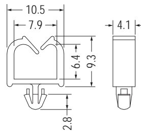
MOUNTING HOLE Ø3.0 THICKNESS 0.8-1.6
