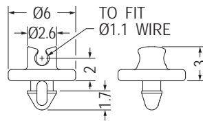
MOUNTING HOLE \varnothing 2.0 THICKNESS 0.8
