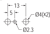
MOUNTING HOLE THICKNESS 0.5-0.8
