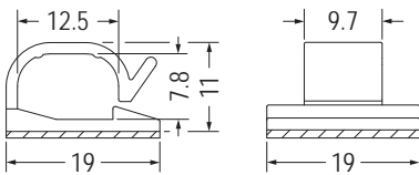
3M DOUBLE ADHESIVE TAPE
