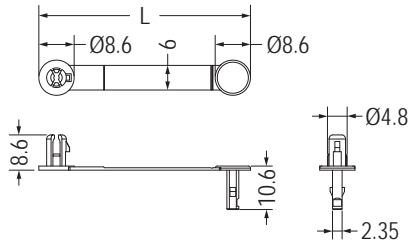
MOUNTING HOLE Ø4.8 THICKNESS: T
