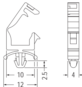
MOUNTING HOLE Ø3.5 THICKNESS 0.8-2.5
