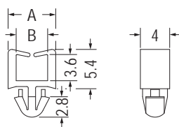
MOUNTING HOLE Ø3.5 THICKNESS: T
