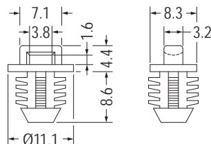
MOUNTING HOLE \varnothing 7.9 THICKNESS 6.4
