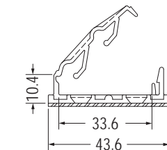
3M DOUBLE ADHESIVE TAPE
