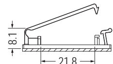
3M DOUBLE ADHESIVE TAPE
