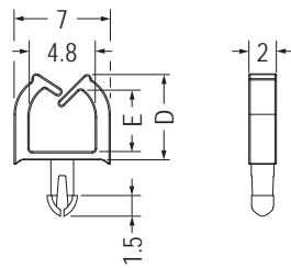
MOUNTING HOLE Ø1.7 THICKNESS: T
