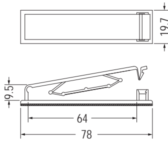
3M DOUBLE ADHESIVE TAPE SUITABLE CABLE 50 PIN
