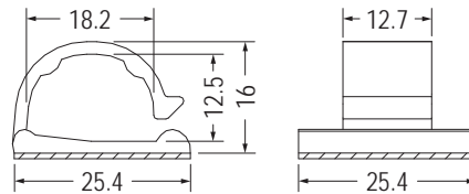
3M DOUBLE ADHESIVE TAPE
