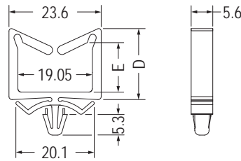
MOUNTING HOLE \varnothing 4.75 THICKNESS 1.2
