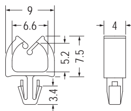
MOUNTING HOLE Ø3.0 THICKNESS 1.6
