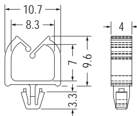
MOUNTING HOLE Ø3.3 THICKNESS 1.0
