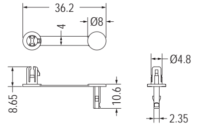
MOUNTING HOLE Ø4.8 THICKNESS 3.5
