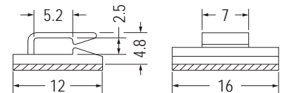
3M DOUBLE ADHESIVE TAPE
