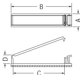
3M DOUBLE ADHESIVE TAPE
