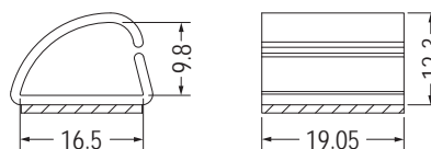
3M DOUBLE ADHESIVE TAPE
