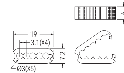
UNIT FOLDED VIEW
