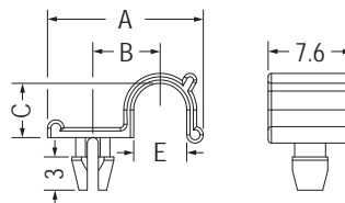
MOUNTING HOLE Ø3.2 THICKNESS 1.6
