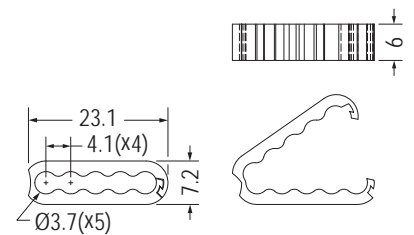
UNIT FOLDED VIEW
