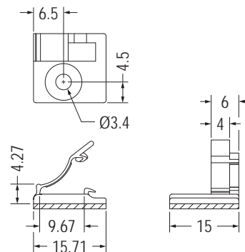
3M DOUBLE ADHESIVE TAPE
