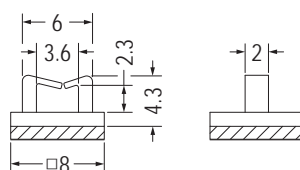
3M DOUBLE ADHESIVE TAPE
