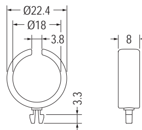
MOUNTING HOLE Ø4.0 THICKNESS 2.5
