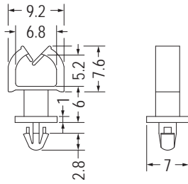
MOUNTING HOLE Ø3.0 THICKNESS 1.0-1.6
