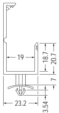
MOUNTING HOLE Ø4.8 THICKNESS 0.8-1.6
