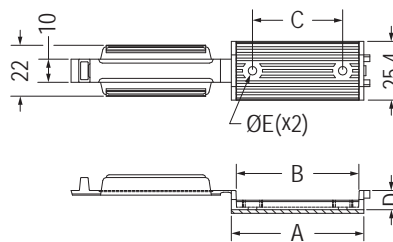
3M DOUBLE ADHESIVE TAPE
