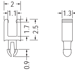
MOUNTING HOLE Ø1.0 THICKNESS 1.0
