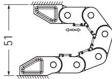
PRINCIPLE SKETCH - BEND RA-DIUS
