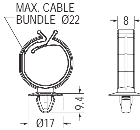
MOUNTING HOLE \varnothing 6.5\text{--}\varnothing 7.0 THICKNESS 0.6~2.0
