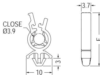
MOUNTING HOLE \varnothing 4.0 THICKNESS 0.8~2.0
