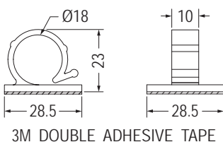
3M DOUBLE ADHESIVE TAPE
