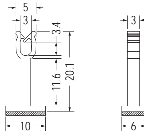
3M DOUBLE ADHESIVE TAPE
