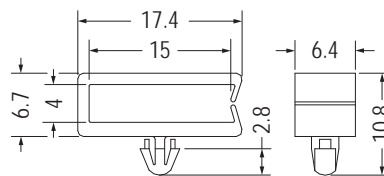
MOUNTING HOLE Ø3.0 THICKNESS 1.0
