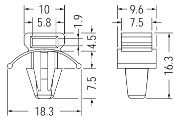
MOUNTING HOLE Ø6.2-Ø6.3 THICKNESS 0.8-3.6
