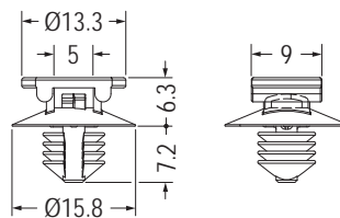
MOUNTING HOLE \varnothing 6.5\text{-}\varnothing 7.0 THICKNESS 0.8-3.0
