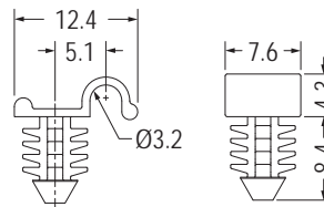
MOUNTING HOLE Ø6.35 THICKNESS 6.35
