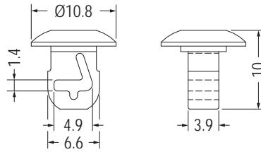
MOUNTING HOLE Ø6.4 THICKNESS 3.2
