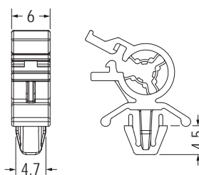
MOUNTING HOLE \varnothing 4.8 THICKNESS 0.5~2.0
