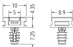
MOUNTING HOLE \varnothing 3.3\text{-}\varnothing 4.0 (M4) THICKNESS 1.0-3.0
