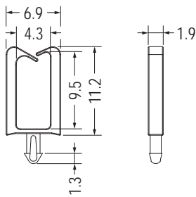
MOUNTING HOLE Ø1.75 THICKNESS 2.2
