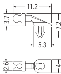
MOUNTING HOLE \varnothing 2.0 THICKNESS 1.6
