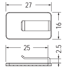
3M DOUBLE ADHESIVE TAPE
