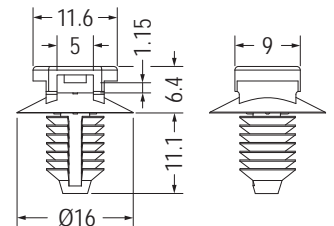
MOUNTING HOLE \varnothing 6.4\text{-}\varnothing 7.1 THICKNESS 0.8-6.0
