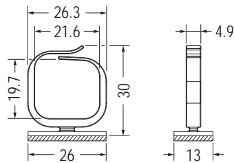
3M DOUBLE ADHESIVE TAPE
