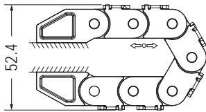
PRINCIPLE SKETCH - BEND RA-DIUS
