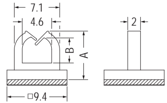
3M DOUBLE ADHESIVE TAPE
