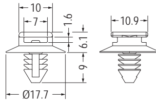
MOUNTING HOLE \varnothing 6.0\text{-}\varnothing 6.4 THICKNESS 0.8-9.0
