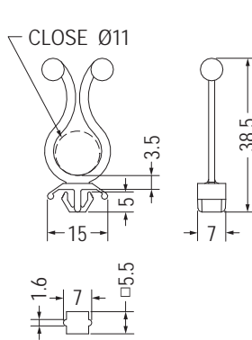
MOUNTING HOLE THICKNESS: 0.8-1.2
