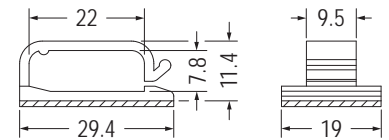
3M DOUBLE ADHESIVE TAPE
