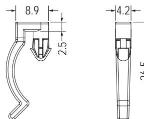
MOUNTING HOLE Ø4.3 THICKNESS 4.0
