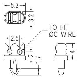
MOUNTING HOLE \varnothing 2.0 THICKNESS: T
