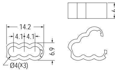
UNIT FOLDED VIEW
