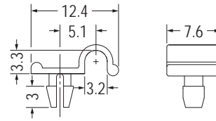
MOUNTING HOLE Ø3.2 THICKNESS 1.6
