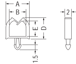
MOUNTING HOLE Ø1.75 THICKNESS 1.6
