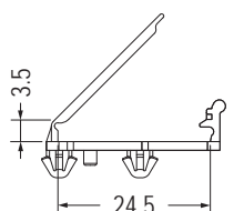
MOUNTING HOLE THICKNESS 0.5-0.8
