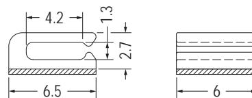
3M DOUBLE ADHESIVE TAPE
