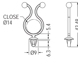
MOUNTING HOLE Ø4.8-Ø5.0 THICKNESS 1.2-2.0
