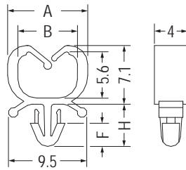
MOUNTING HOLE Ø3.0 THICKNESS 0.6-1.6
