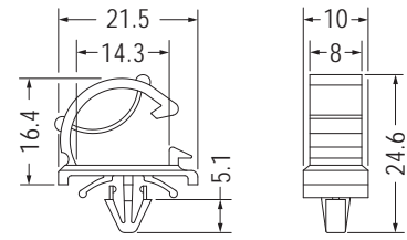
MOUNTING HOLE \varnothing 4.8 THICKNESS 0.8-2.5
