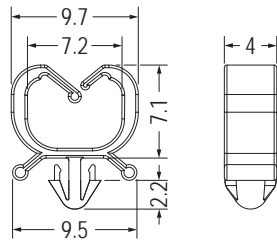
MOUNTING HOLE THICKNESS 0.6-0.8
