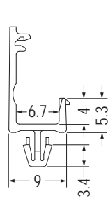
MOUNTING HOLE Ø3.0 THICKNESS 1.2-1.7
