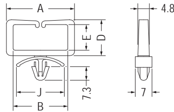
MOUNTING HOLE \varnothing 4.8\text{-}\varnothing 5.0 THICKNESS: T
