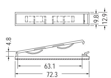
3M DOUBLE ADHESIVE TAPE
