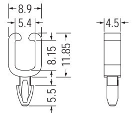
MOUNTING HOLE Ø4.0 THICKNESS 2.2
