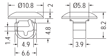
MOUNTING HOLE Ø6.4 THICKNESS 1.3
