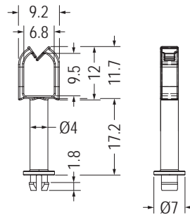
MOUNTING HOLE Ø3.8 THICKNESS 1.7
