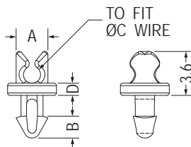
MOUNTING HOLE: \varnothing G THICKNESS: T
