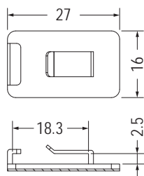
3M DOUBLE ADHESIVE TAPE
