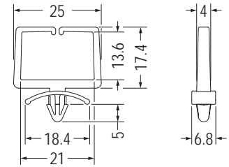
MOUNTING HOLE \varnothing 4.8\text{-}\varnothing 5.0 THICKNESS 0.8-2.5
