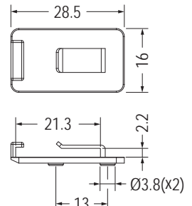
3M DOUBLE ADHESIVE TAPE
