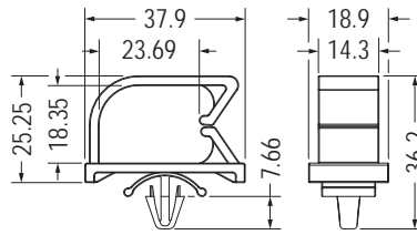
MOUNTING HOLE Ø6.4 THICKNESS 1.9
