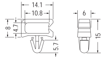
MOUNTING HOLE Ø4.8 THICKNESS 0.8-1.6
