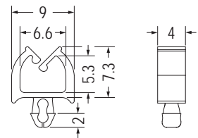
MOUNTING HOLE Ø3.0 THICKNESS 1.2-1.6
