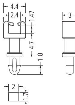
MOUNTING HOLE Ø1.5 THICKNESS 1.5
