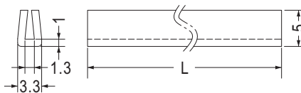
CHASSIS THICKNESS 0.8~1.2
