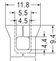
CLOSE PART
