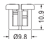
MOUNTING HOLE \varnothing 9.5 THICKNESS 0.6~3.2
