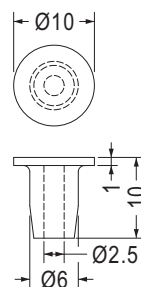
MOUNTING HOLE Ø5.5~Ø5.8
