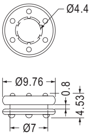
MOUNTING HOLE Ø7.0~Ø7.5
