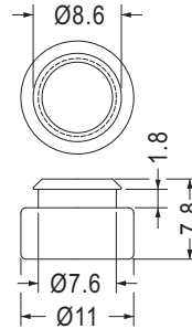
MOUNTING HOLE Ø7.0~Ø7.3 THICKNESS 1.0~1.5
