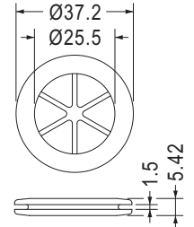
MOUNTING HOLE Ø28.5
