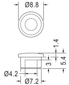
MOUNTING HOLE Ø7.0
