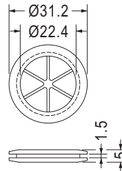
MOUNTING HOLE Ø25.4
