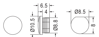
MOUNTING HOLE
