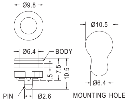
裝配孔尺寸，僅供參考 Mounting holes are for reference only.
