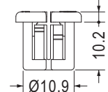
MOUNTING HOLE \varnothing 11.1 THICKNESS 0.6~3.2
