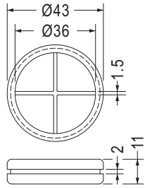
MOUNTING HOLE Ø40.0 THICKNESS 2.0
