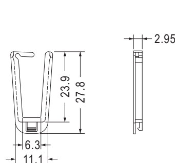
MOUNTING HOLE THICKNESS 1.0
