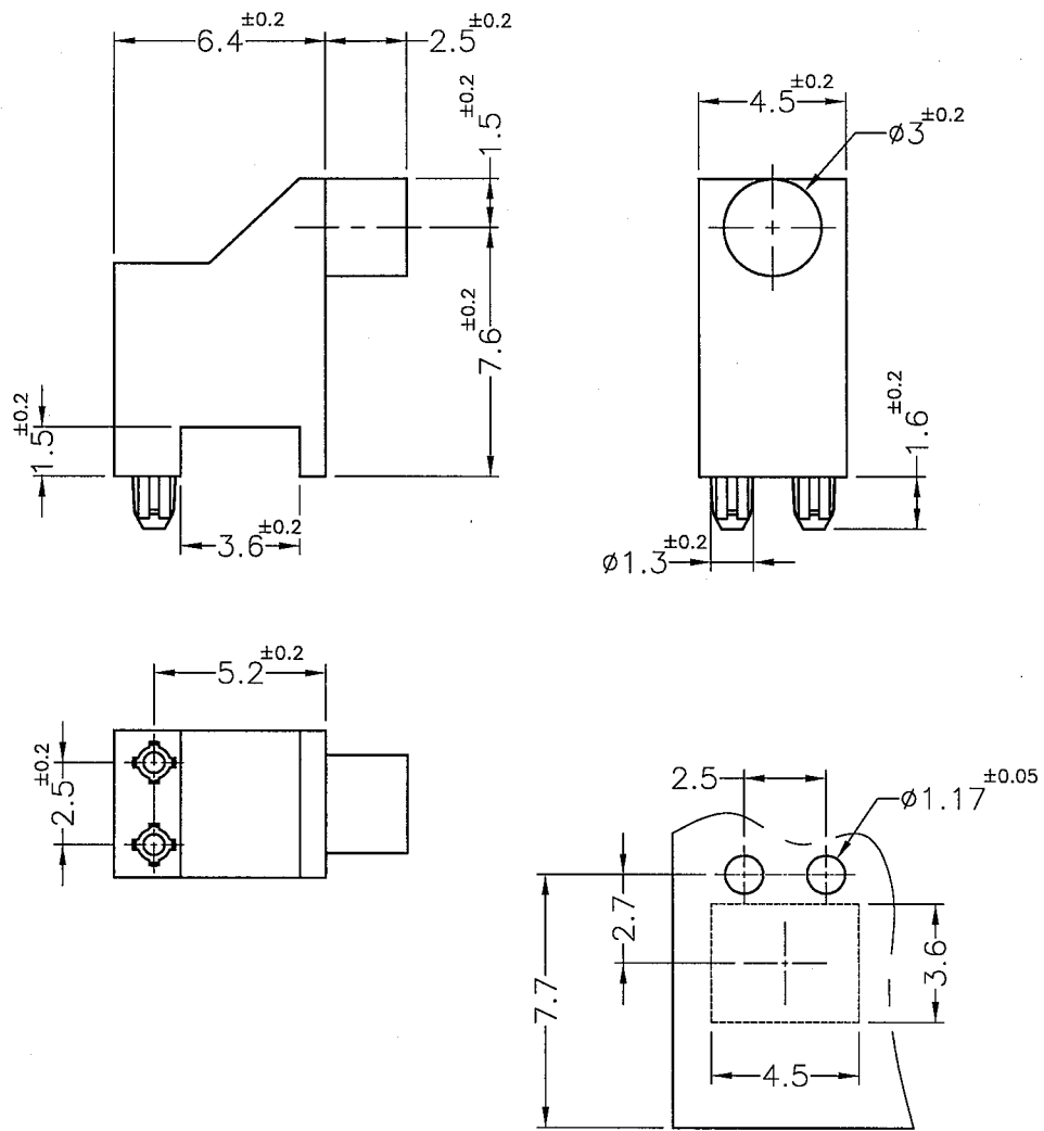
MOUNTING HOLE (RECOMMEND FOR REFERENCE ONLY)
