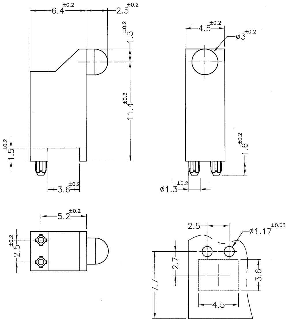
MOUNTING HOLE (RECOMMEND FOR REFERENCE ONLY)
