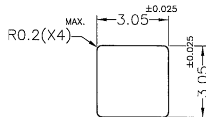
MOUNTING HOLE (RECOMMEND FOR REFERENCE ONLY)
