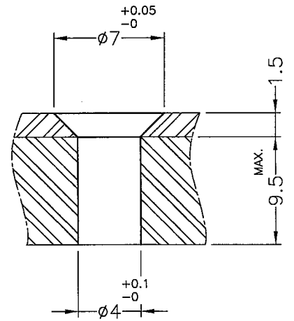
MOUNTING HOLE (RECOMMEND FOR REFERENCE ONLY)
