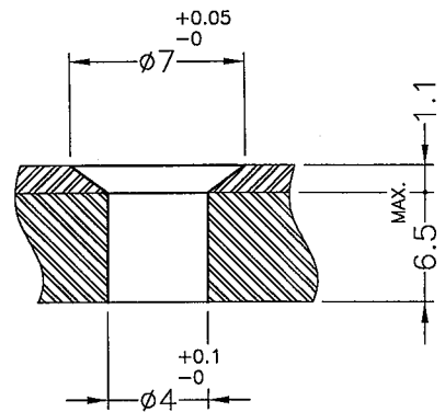
MOUNTING HOLE (RECOMMEND FOR REFERENCE ONLY)
