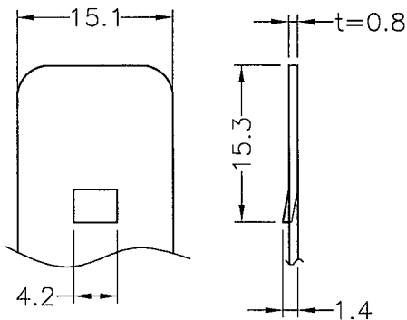
ASSEMBLY PART (裝配件尺寸, 僅供參考)
