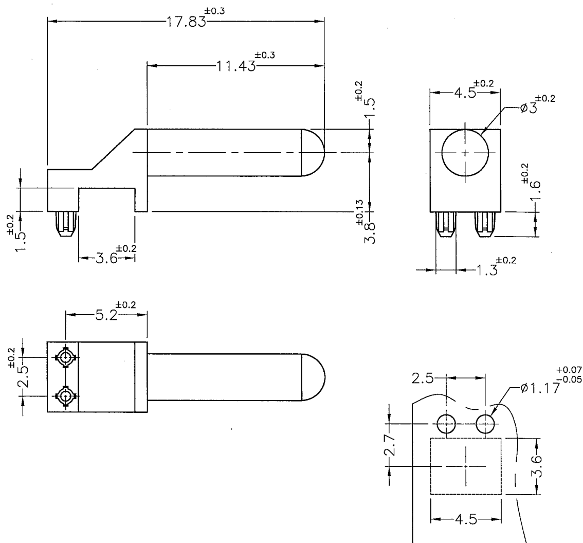
MOUNTING HOLE (RECOMMEND FOR REFERENCE ONLY)
