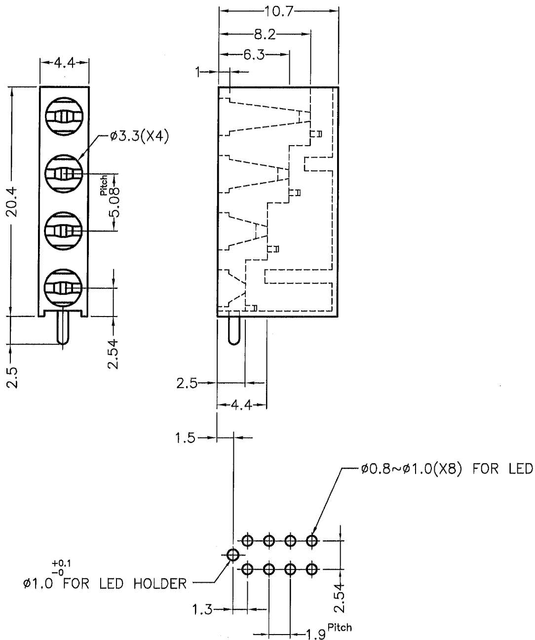
MOUNTING HOLES
