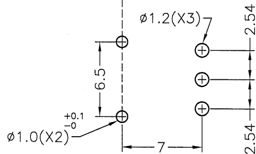
3PIN LED MOUNTING HOLES
