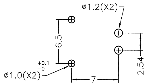
2PIN LED MOUNTING HOLES
